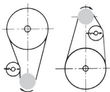
Vertical Centerlines
